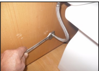
10 – Turn on the water Proceed to two discharges Check for water leaks
